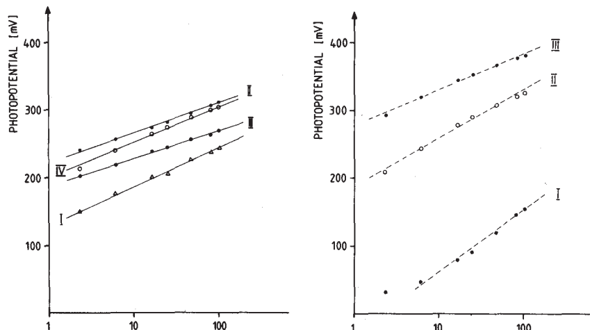
Fig. 3. Photopotentials of sintered iron(III) oxide in different electrolytes versus the relative light intensity. Left, 1% \text{SnO}_2 ; right 1% \text{CaO} .
