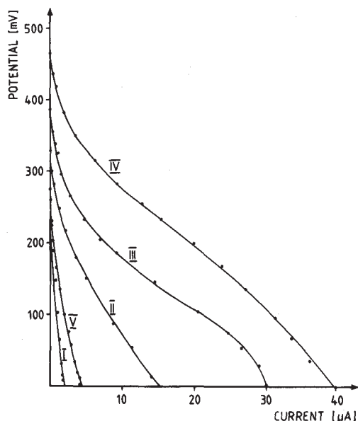
Fig. 5. Current-voltage characteristics for the different electrolytes given in Table 1. Doping: 1% CaO. I and II with a 300 W xenon lamp. III, IV, V with a 150 W xenon lamp.
