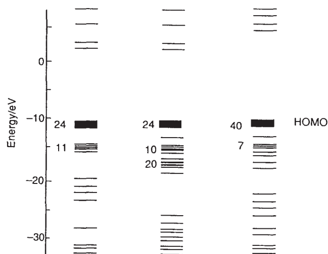
Fig. 11 MO level diagram. From left to right: \text{H}_8\text{Si}_8\text{O}_{12} , (\text{CH}_3)_8\text{Si}_8\text{O}_{12} , and \text{Cl}_8\text{Si}_8\text{O}_{12} . The numbers indicate the number of levels in the corresponding region
