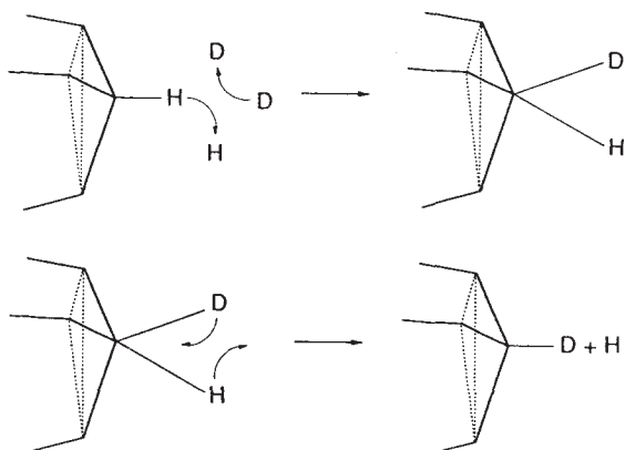
Scheme 15
