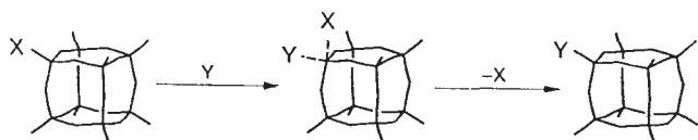
Scheme 17
