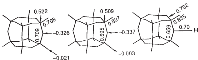
Fig. 13 Overlap population and charge distribution in: (\text{CH}_3)_8\text{Si}_8\text{O}_{12} , left; \text{H}_8\text{Si}_8\text{O}_{12} , middle; and [\text{H}_9\text{Si}_8\text{O}_{12}]^+ , right. The numbers without arrows indicate the overlap populations, the others represent charges. For [\text{H}_9\text{Si}_8\text{O}_{12}]^+ only overlap populations are shown
