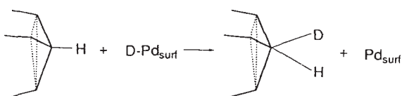
Scheme 16
