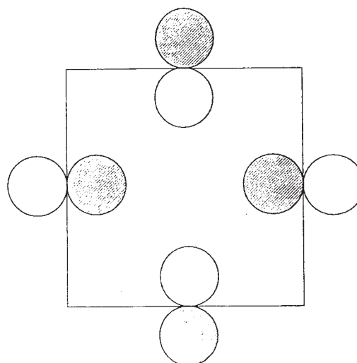
Scheme 9
