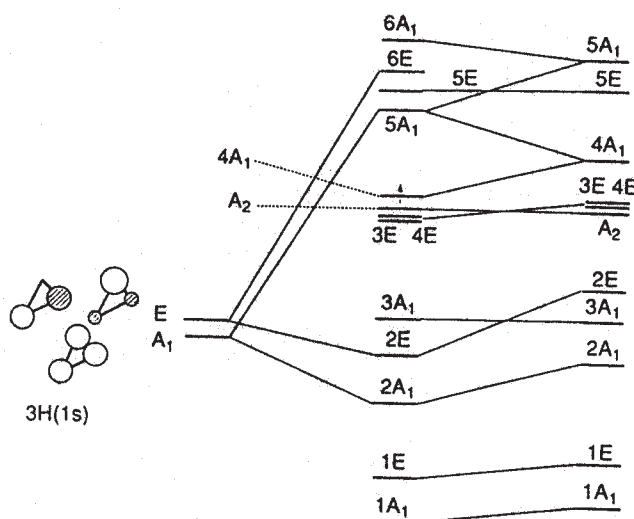
Fig. 2 Correlation diagram for 3\text{H} + \text{O}_3\text{Si} \rightarrow (\text{HO})_3\text{Si} . The 4A_1 orbital of (\text{HO})_3\text{Si} is occupied by one electron
