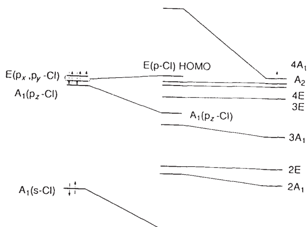
Fig. 7 Correlation diagram for (\text{HO})_3\text{Si} + \text{Cl} \rightarrow (\text{HO})_3\text{Si-Cl}
