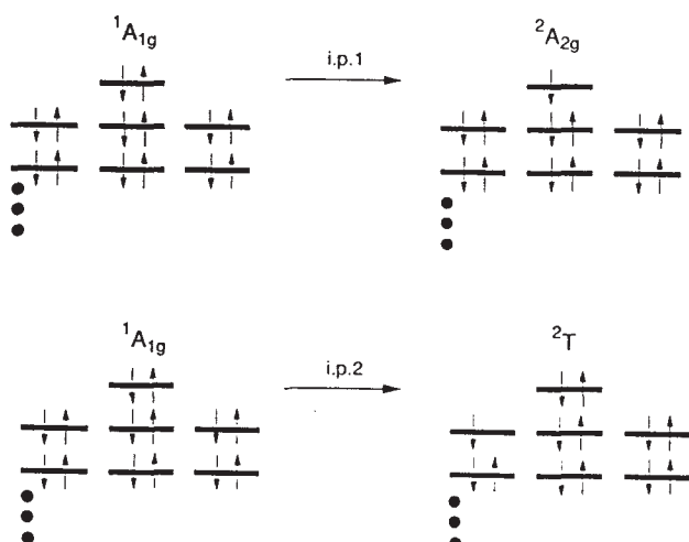
Scheme 10
