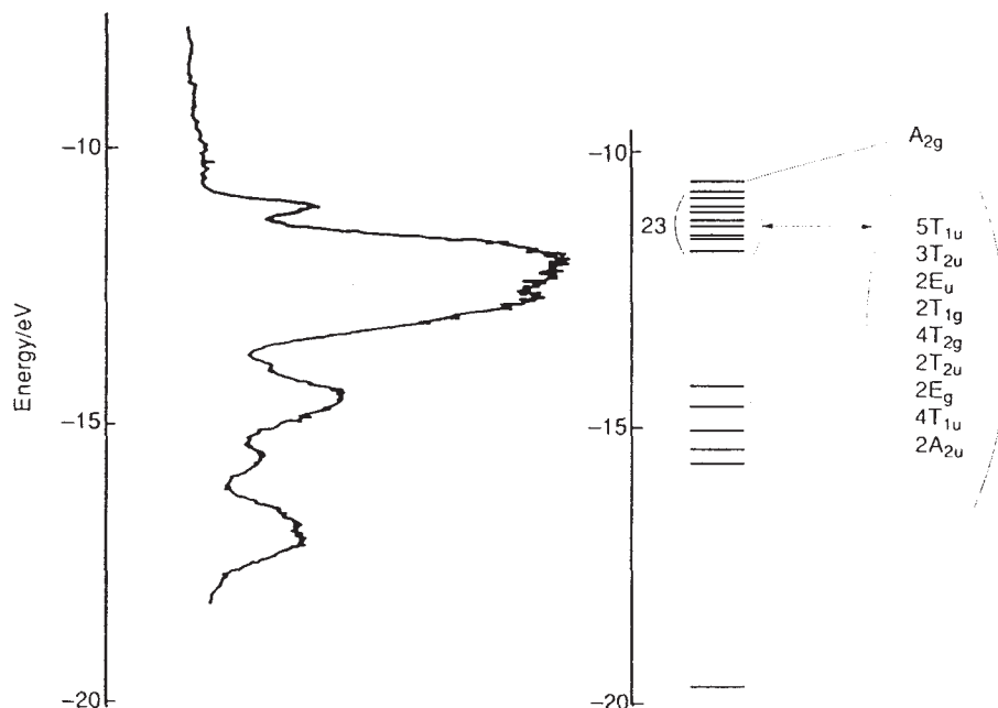
Fig. 12 Photoelectron spectrum of \text{H}_8\text{Si}_8\text{O}_{12} 26 (left) and calculated one-electron levels (right)
