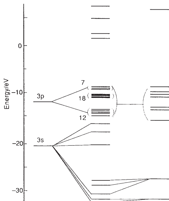
Fig. 10 Correlation diagram. The numbers indicate the number of levels in the corresponding region. Left: 4\text{Si} + 4\text{SiO}_3 \rightarrow \text{Si}_8\text{O}_{12} . Right: the region between -15 and -9 eV magnified. Correlation with the 3p AOs of Si and the 2p AOs of O is shown
