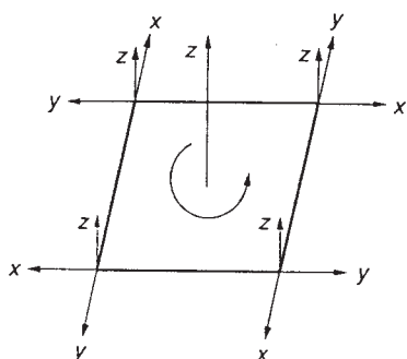
Scheme 8
