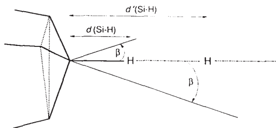
Scheme 12
