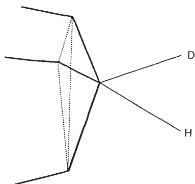
Scheme 14
