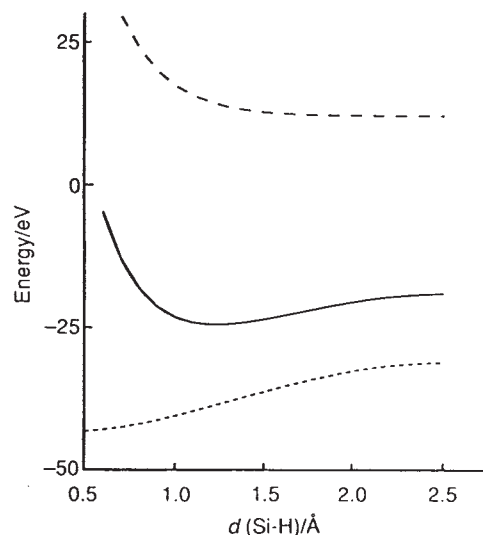
Fig. 4 The Si-H stretching mode of SiH(OH)_3 . (-----) Two-body interaction E_{\alpha\beta}(R) , (.....) \Delta E_{EHMO}(R) , (—) \Delta E_{EHMO}(R) + E_{\alpha\beta}(R)
